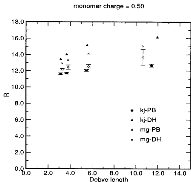
FIG. 2. Same as Fig. 1 for monomer charge 0.50. The Debye lengths, in decreasing order, correspond to one, 20, 50, and 70 monovalent impurity ion pairs.
