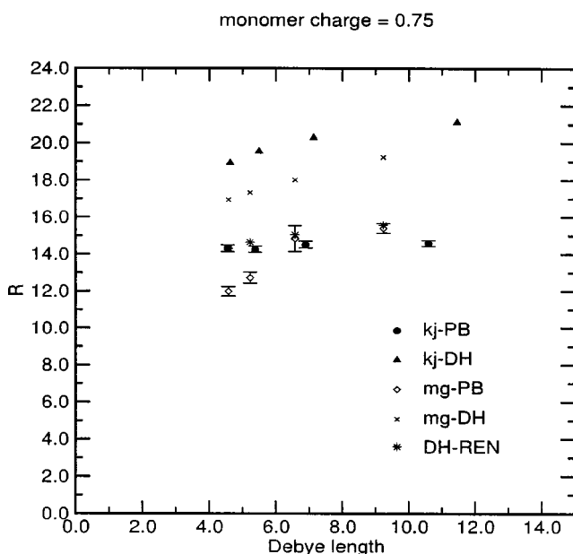
FIG. 3. Same as Fig. 1 for monomer charge 0.75. The Debye lengths, in decreasing order, correspond to one, ten, 20, and 30 monovalent impurity ion pairs. DH-REN indicates results of a simulation based on a Debye–Hückel pair potential with renormalized monomer charge; see text for details. (It should be noted that the results for kj-PB and DH-REN in the case of 30 monovalent impurity ions are nearly coincident.)
