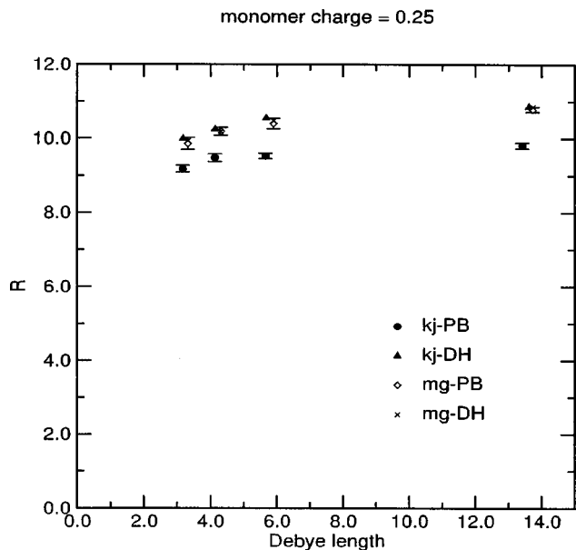
FIG. 1. The end-to-end distance R as a function of Debye length, both in units of bond length (4 Å), for a chain of 32 monomers, each having a charge of 0.25 (in units of the proton charge). The Debye lengths are averaged over the course of the simulation, and, in decreasing order, correspond to one, 20, 40, and 70 monovalent impurity ion pairs plus the appropriate number of monovalent negative counterions needed for electroneutrality of the solution; see text for further details. (The error bars for the Debye lengths, as well as for the Debye–Hückel results, are negligible and are, therefore, not shown.) The swelling of the chains due to the electrostatic repulsion between the charged monomers is evident, in comparison to the uncharged case for which R \cong 7.85 . In the legend “kj” stands for results of the KJMC method, “mg” stands for the results of the multigrid CBMC techniques, “PB” stands for Poisson–Boltzmann, and “DH” stands for Debye–Hückel.
